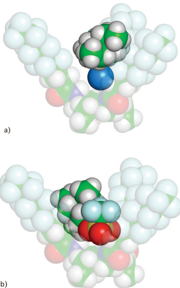
FIGURE 3. (a) DFT-optimized view of 3 •TEACl, showing the counteraction inside of the binding pocket. The N_{\text{TEA}} \cdots \text{Cl}^- separation is 4.21 Å, and the average \text{NH} \cdots \text{Cl}^- hydrogen-bond length is 2.99 Å. (b) DFT-optimized view of 3 •TEACF 3 SO 3 , showing the counteraction outside of the binding pocket. The N_{\text{TEA}} \cdots \text{S}_{\text{triflate}} separation is 6.42 Å, the closest N_{\text{TEA}} \cdots \text{O}_{\text{triflate}} approach is 5.52 Å, and the average \text{NH} \cdots \text{O}_{\text{triflate}} hydrogen-bond length is 2.16 Å.
